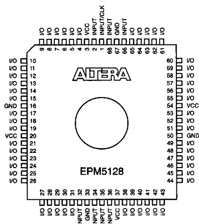
J-Lead
