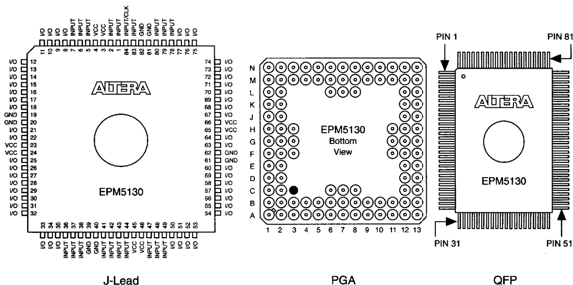
Figure 21. EPM5130 Package Pin-Out Diagrams
