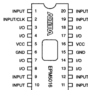
DIP
