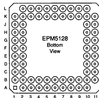
PGA
