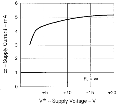
SUPPLY CURRENT
