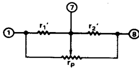
Figure 1. High Resolution, High Stability Nulling Circuit
