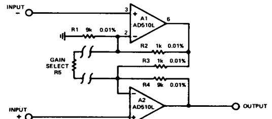
Figure 2. Instrumentation Amplifier
