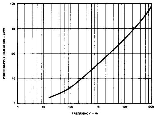
Figure 4. PSRR vs. Frequency
