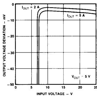
Line Regulation
