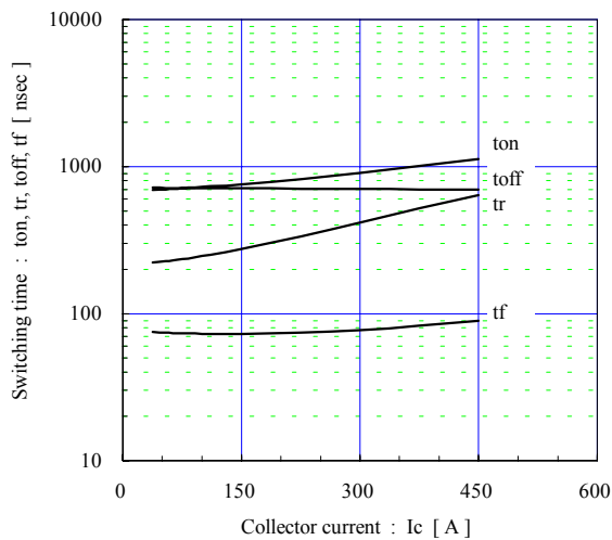
Switching time vs. Collector current (typ.) V_{cc}=300V, V_{GE}=\pm 15V, R_g=9.1\Omega, T_j=125^\circ C
