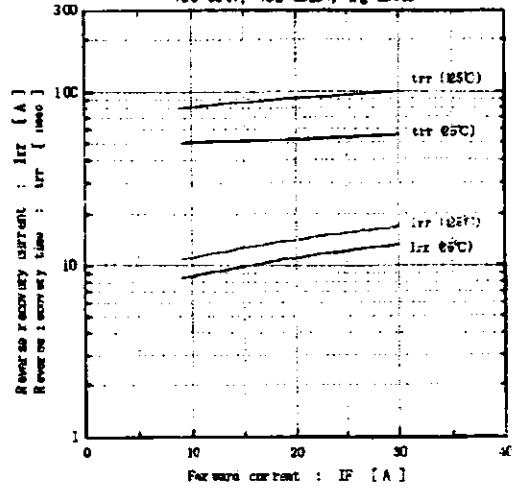
[ Inverter ] Reverse recovery characteristics (typ.) V_C = 300V, V_{GB} = \pm 15V, R_g = 120\Omega
