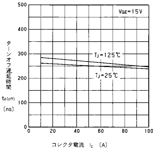
t_{d(off)} - I_C Characteristics t_{d(off)} - I_C Characteristics
