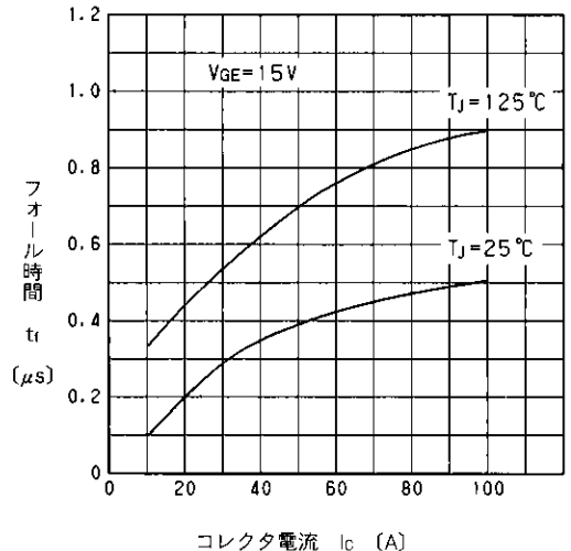
t_r - I_C Characteristics t_r - I_C Characteristics
