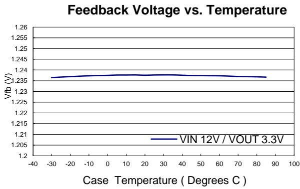
Figure 7. Feedback Voltage vs. Temperature
