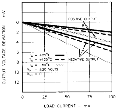
FIGURE 1. LOAD REGULATION
