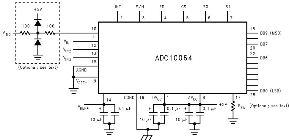
FIGURE 4. Typical Connection
