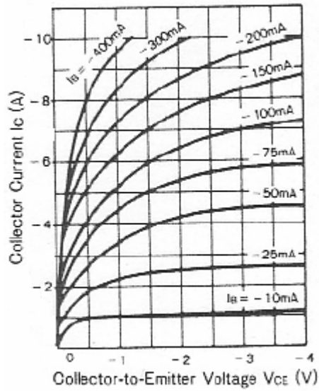
Fig.3 Static Characteristic
