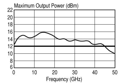
83051A Amplifier
