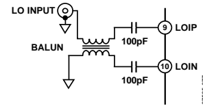
Figure 80. Differential LO Drive
