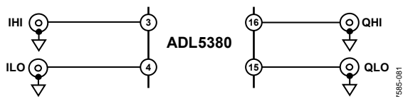
Figure 85. Baseband Output Configuration
