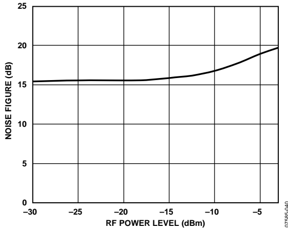
Figure 40. Noise Figure vs. Input Blocker Level, f_{LO} = 5800 MHz (RF Blocker 5 MHz Offset)
