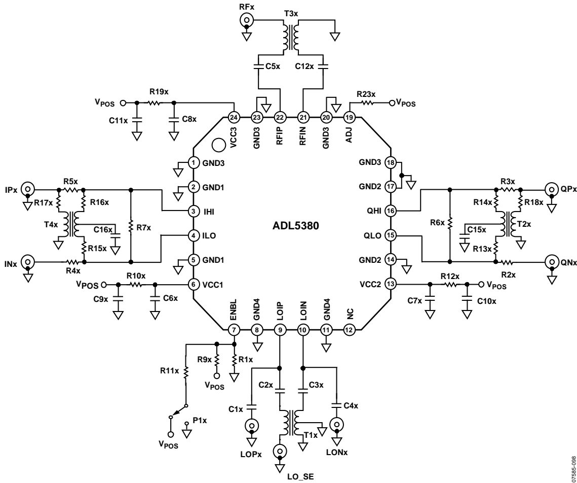
Figure 102. Evaluation Board Schematic
