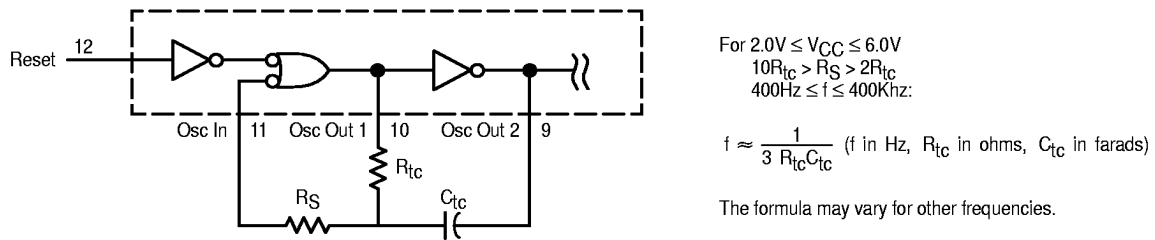
Figure 6. Oscillator Circuit Using RC Configuration
