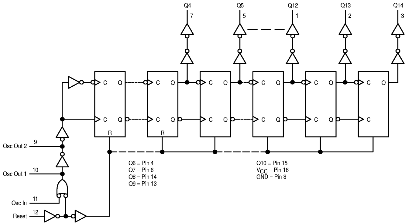
Figure 5. Expanded Logic Diagram
