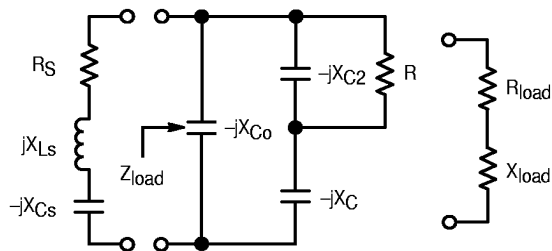
Figure 9. Series Equivalent Crystal Load
