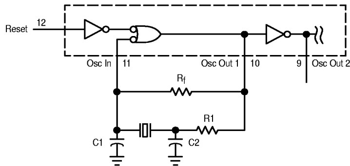
Figure 7. Pierce Crystal Oscillator Circuit
