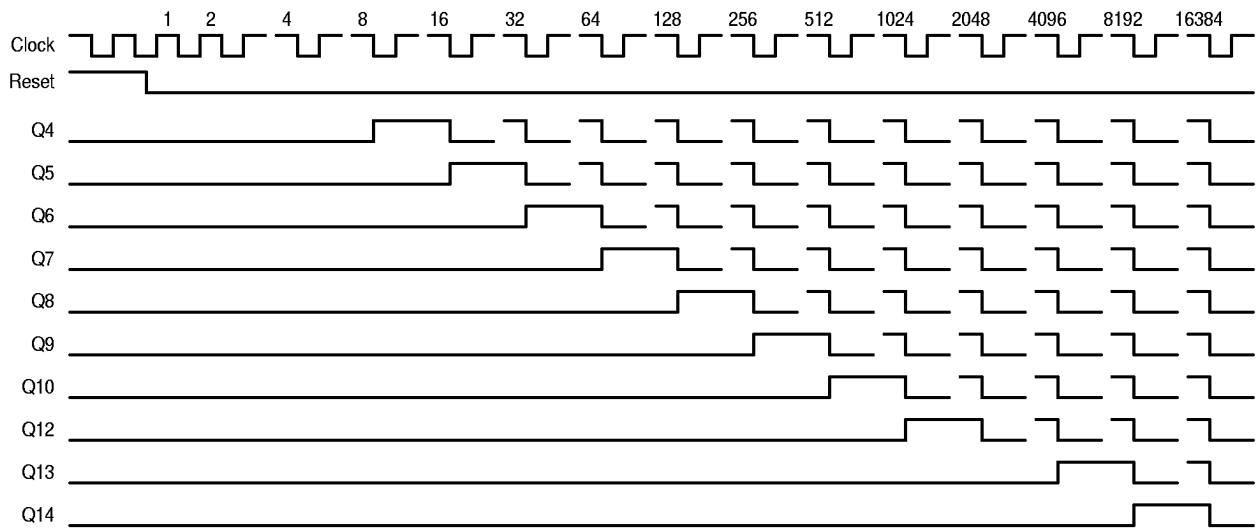
Figure 11. Timing Diagram
