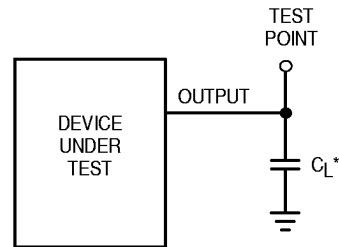
Figure 4. Test Circuit
