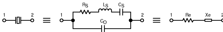
Figure 8. Equivalent Crystal Networks
