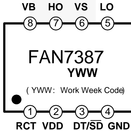
Figure 6. Pin Configurations (Top View)
