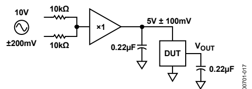
Figure 17. Ripple Rejection Test Circuit
