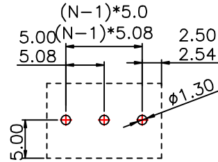
PCB LAYOUT(RECOMMENDED)
