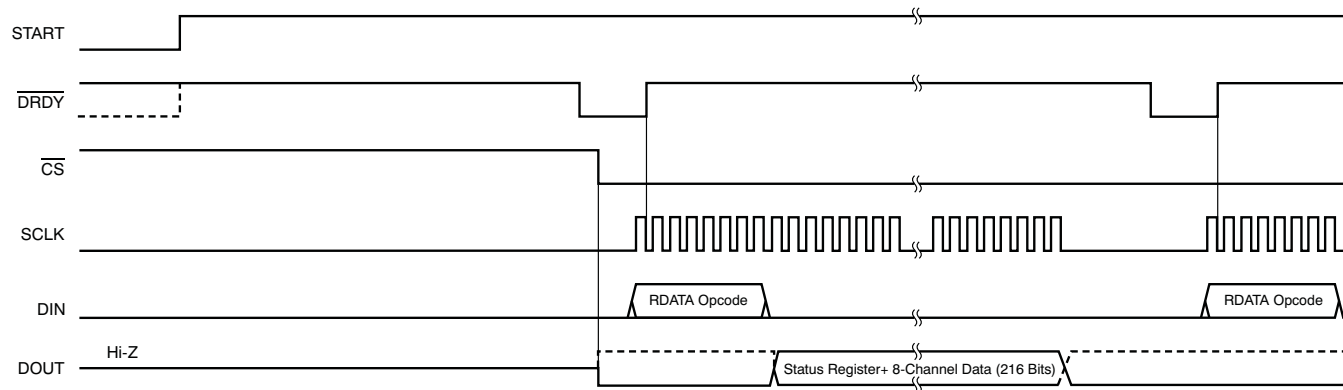
Figure 42. RDATA Usage
