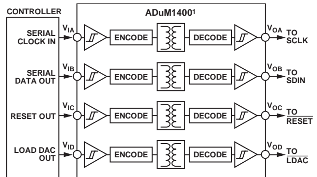
Figure 51. Isolated Interface
