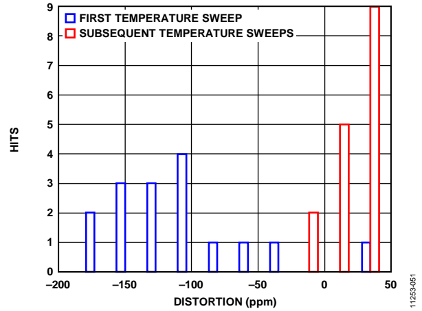
Figure 48. Thermal Hysteresis
