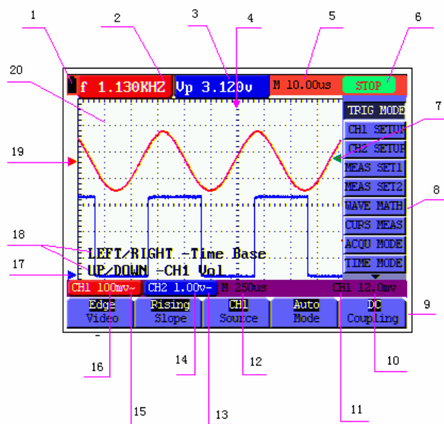
figure 4: Oscilloscope Operation Window
