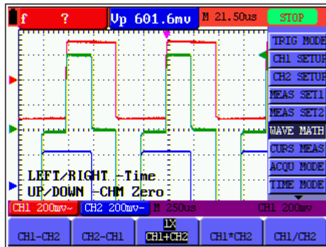
figure 19: Waveform Mathematics
