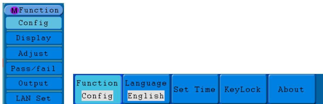
Figure 5-39 Configuration Menu
