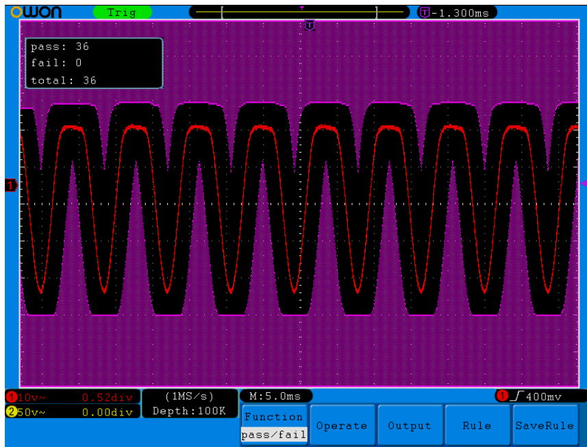
Figure 5-44 Pass/Fail test
