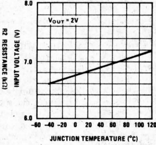
Minimum Input Voltage vs Junction Temperature
