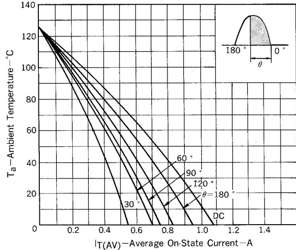
Fig. 4 T_a-I_{T(AV)} RATINGS
