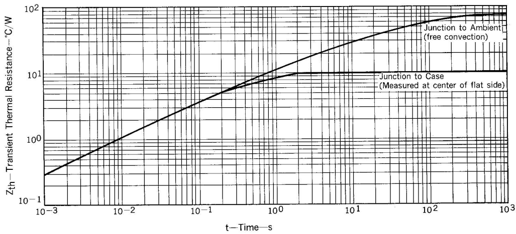
Fig. 11 Z_{th} CHARACTERISTICS
