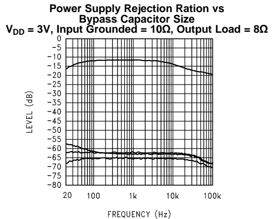
Figure 37. Top Trace = No Cap, Next Trace Down = 1µf Next Trace Down = 2µf, Bottom Trace = 4.7µf
