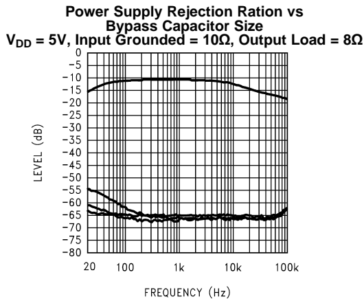
Figure 36. Top Trace = No Cap, Next Trace Down = 1µf Next Trace Down = 2µf, Bottom Trace = 4.7µf
