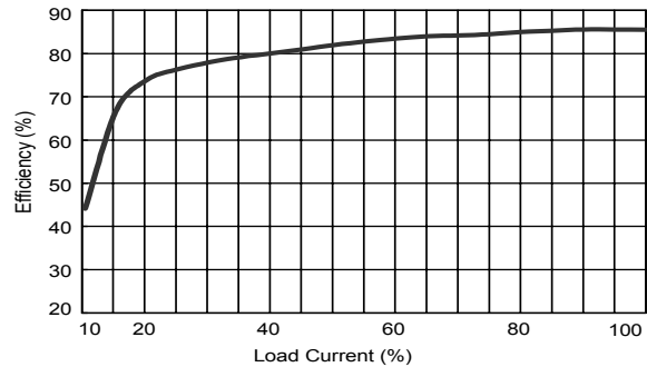
Efficiency vs Output Load ( Dual Output )
