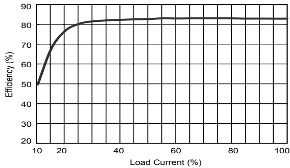
Efficiency vs Output Load ( Single Output )
