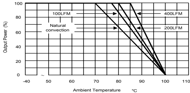
Derating Curve
