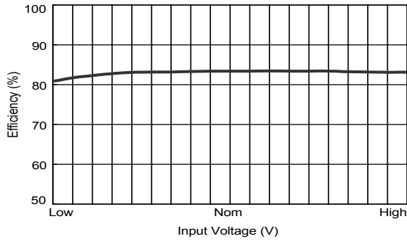
Efficiency vs Input Voltage ( Single Output )
