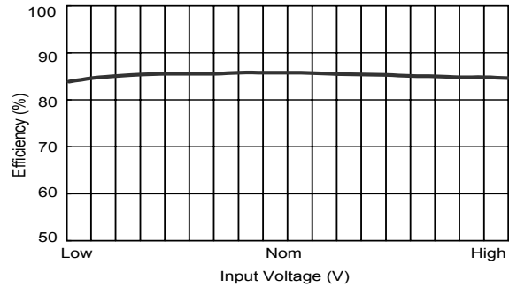
Efficiency vs Input Voltage ( Dual Output )
