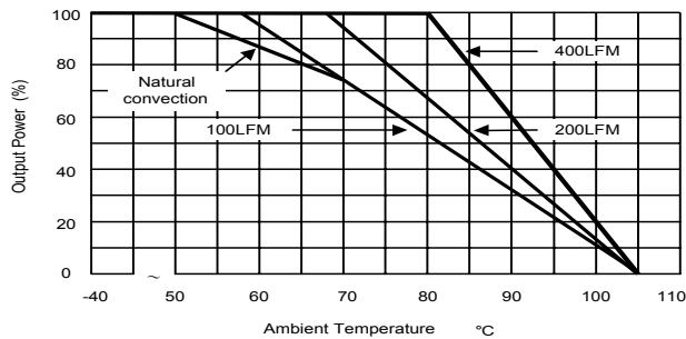
Derating Curve
