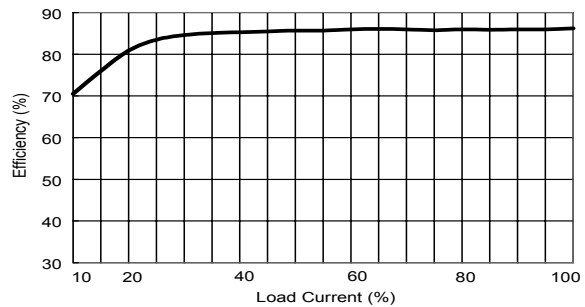
Efficiency vs Output Load ( Dual Output )
