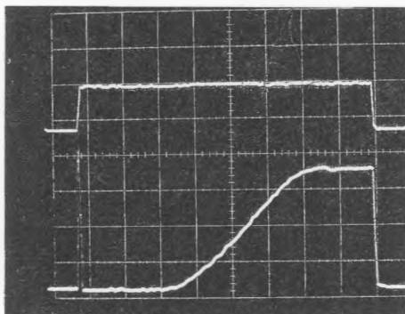
Figure 14 : Current limiting ( V_s = 50V , R_L = 100\Omega ). X = 0.2ms/div. Y = 80mA/div. Upper Trace : command pulse. Lower Trace : load current.
