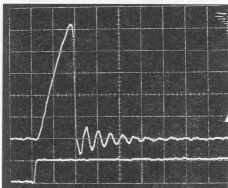
Figure 13 : Current spike ( R_L = 100\Omega , V_s = 50V ). X = 0.5μs/div. Y = 60mA/div. Upper Trace : load current. Lower Trace : command pulse.
