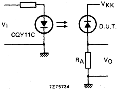
Fig. 2. Switching circuit.
