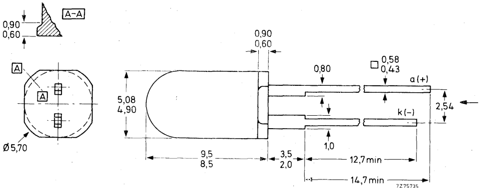
Fig. 1 SOD-39C.
