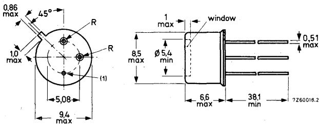
Fig. 1 TO-5 (except for window).
