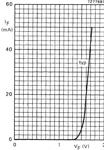
Fig. 6 T_j = 25^{\circ}\text{C} .
