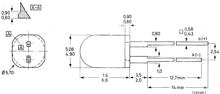
Fig. 1 SOD-39D
