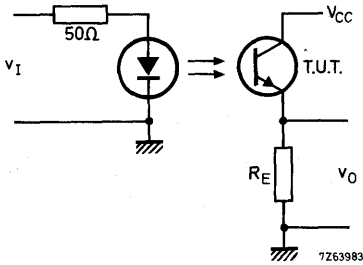
Fig. 2 Switching circuit.
