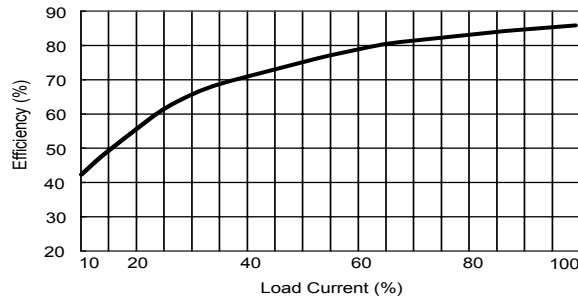
Efficiency vs Output Load ( Dual Output )
