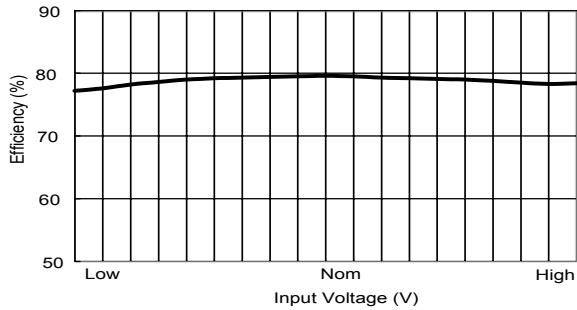
Efficiency vs Input Voltage ( Single Output )
