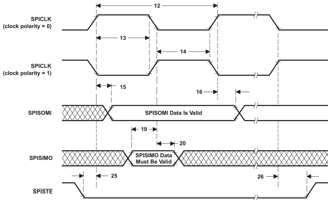
Figure 5-76. SPI Slave Mode External Timing (Clock Phase = 0)
