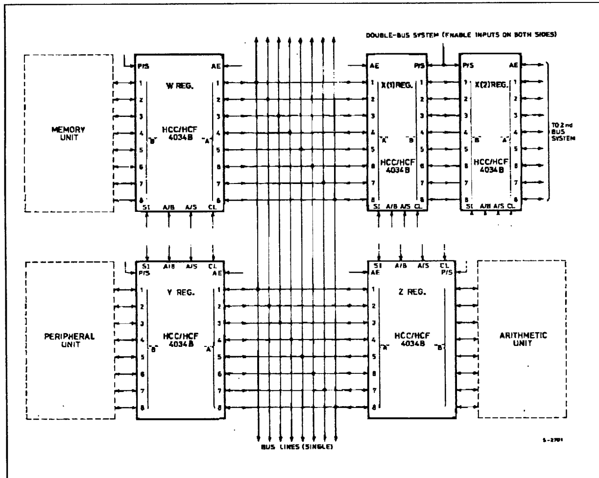
The "A" enable (AE) and A/B signals control all combinations of transfer between the registers and bus systems.
